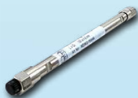
Phenyl
