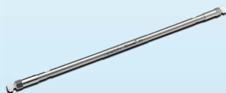
C18
